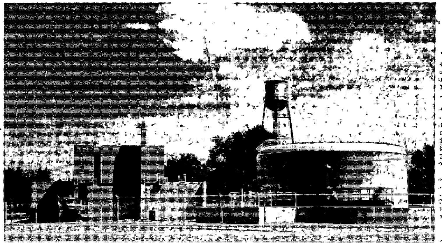
Water plant, clarifier (lower right) and 400,000 gallon ground tank.
