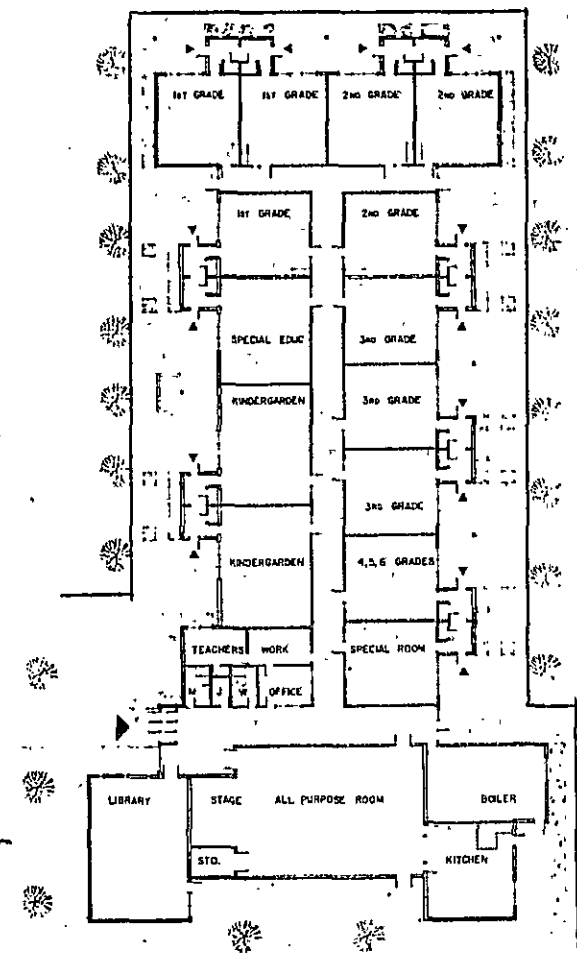
SCHEMATIC FLOOR PLAN
