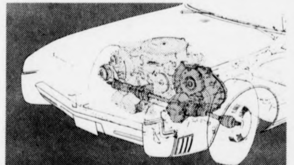
Another first from Oldsmobile! Toronado, only full-size car with front wheel drive! Engine, transmission, differential and steering are all up front... to put the traction where the action is!
