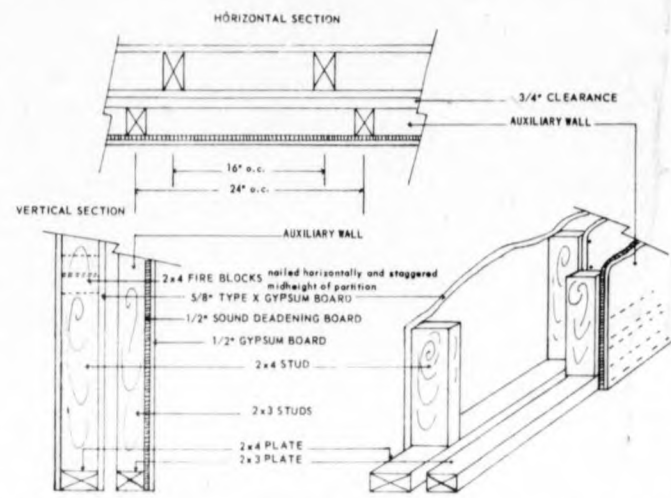
NOISE BETWEEN ROOMS CAN BE REDUCED with this auxiliary wall which can be installed next to the present wall, according to a plan developed by the Insulation Board Institute. A special IBI-rated sound-deadening insulation board controls flow of sounds.
