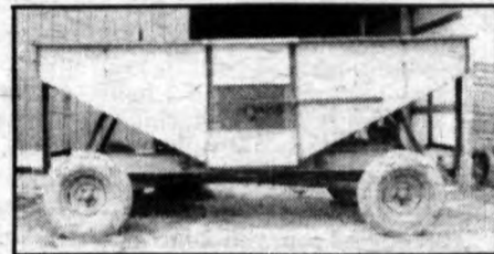
2 - 125 Bu. Gravity Grain Wagons with Running Gear
