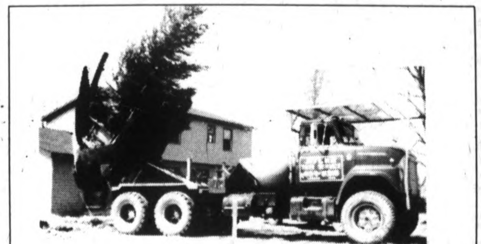
This special large spade can handle trees up to 12" in diameter.
