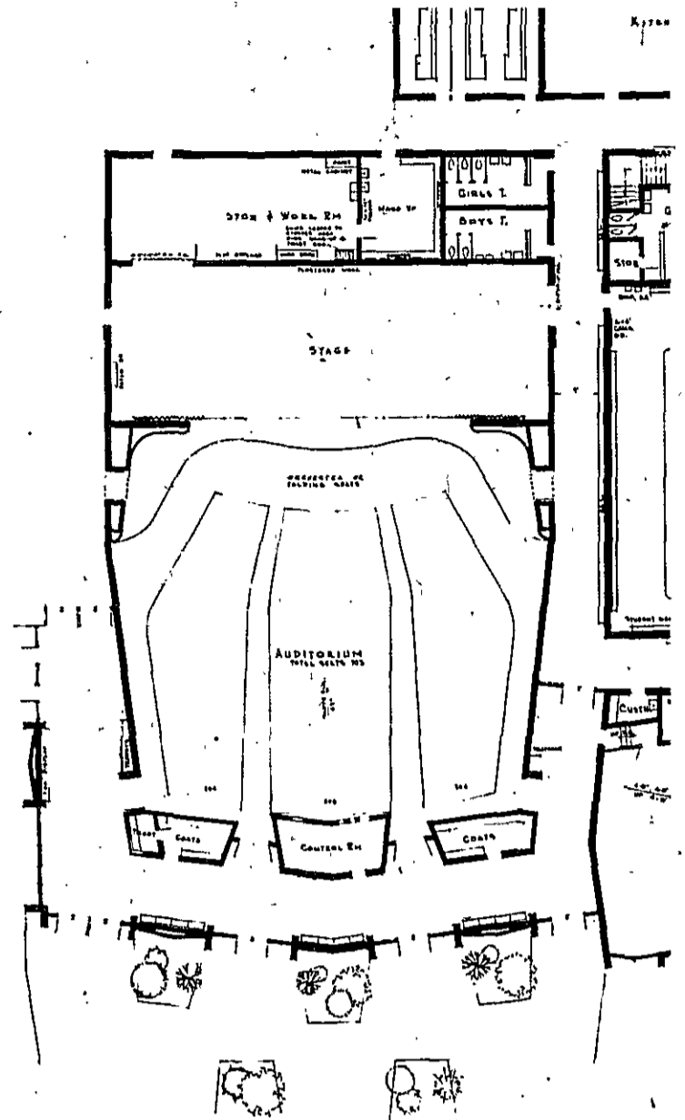
This is a detailed close-up of the auditorium, stage, storage and workroom, and make-up room at the new St. Johns High School now under construction. The stage itself is about four times as large as the stage in the present high school.
